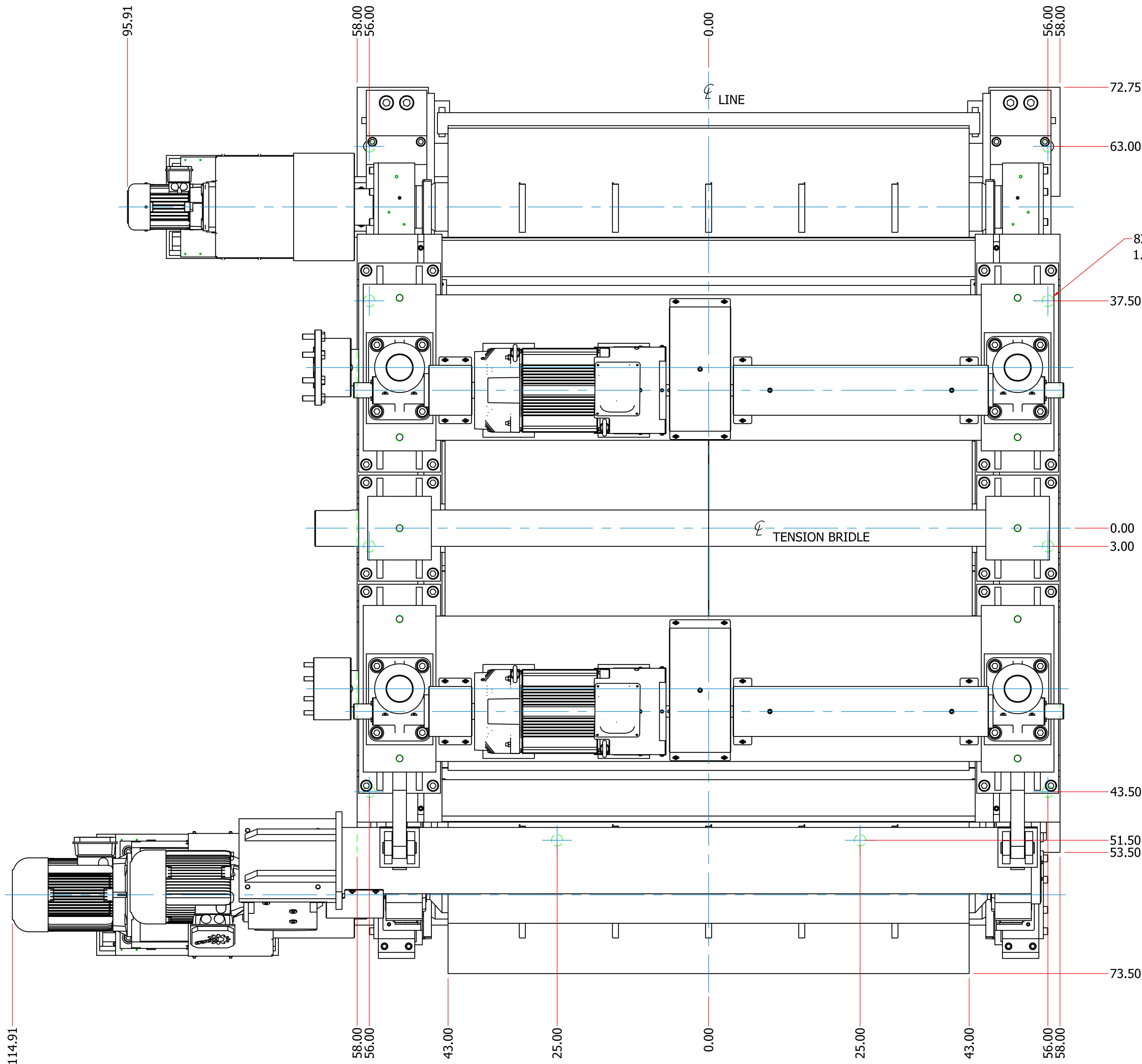
VIEW A-A SCALE 1" = 1'
