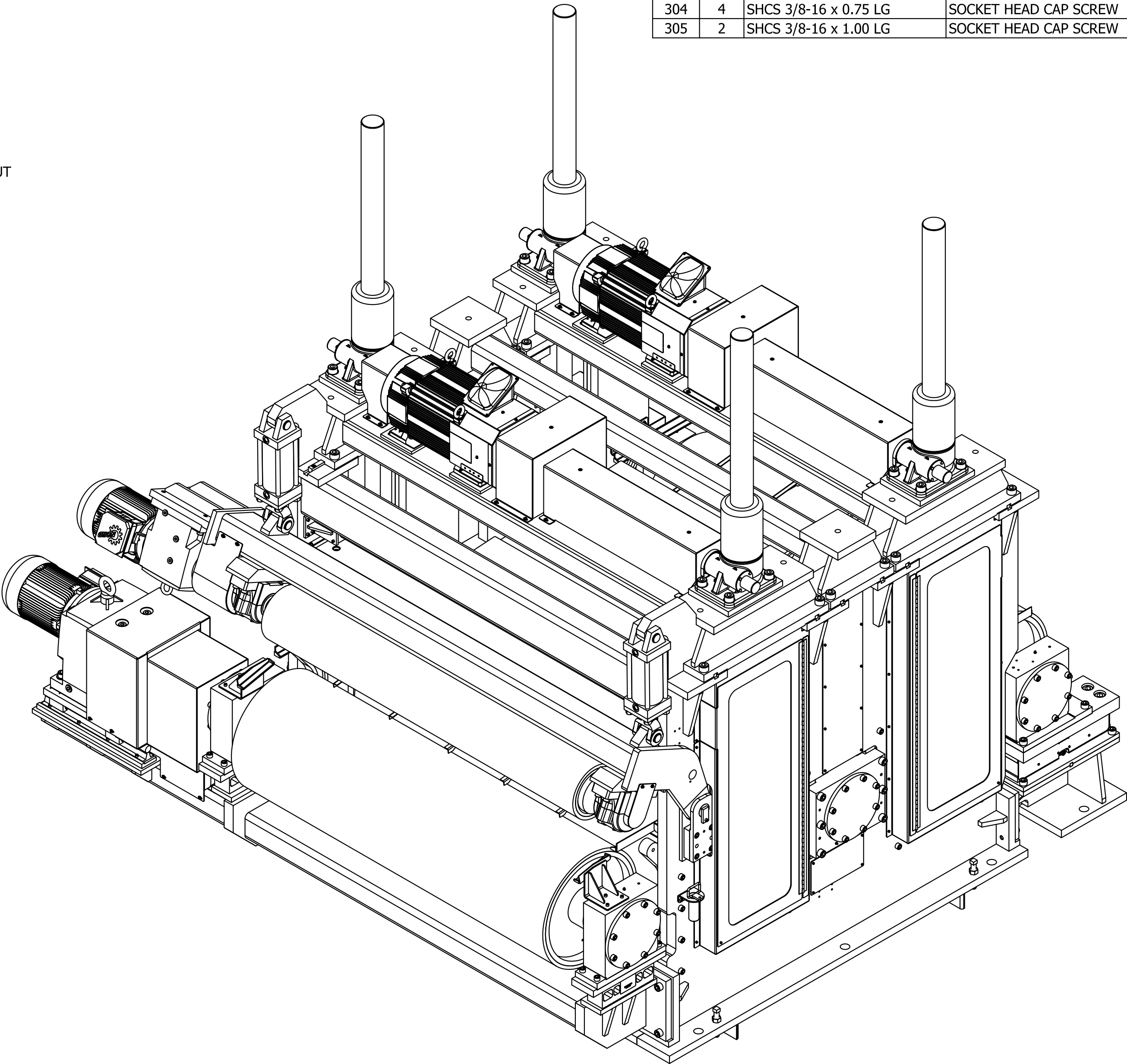
ISOMETRIC VIEW SCALE 3/4" = 1'
