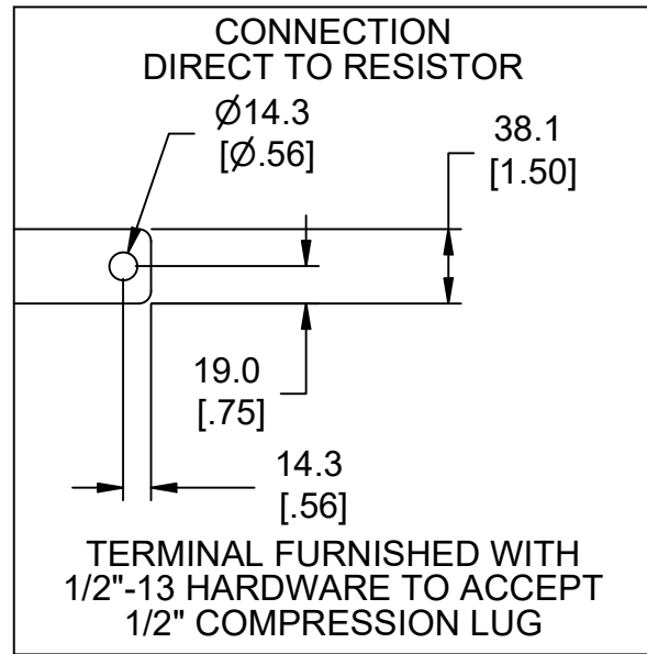
DETAIL FOR NEUTRAL
