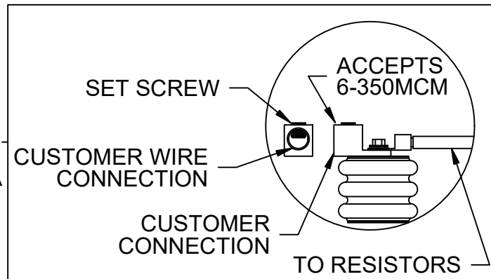
DETAIL FOR GROUND CONNECTION
