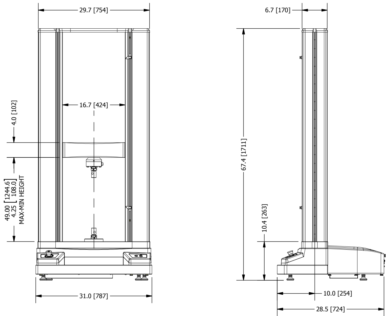
30kN Load Capacity Series Test Frames
