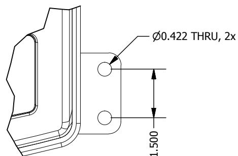
Bench Clip Hole Pattern
