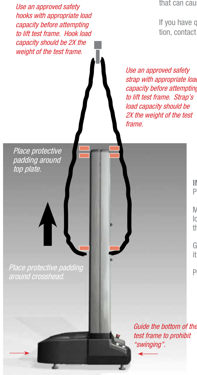
Lifting the MMD/FMD Series using a crane
