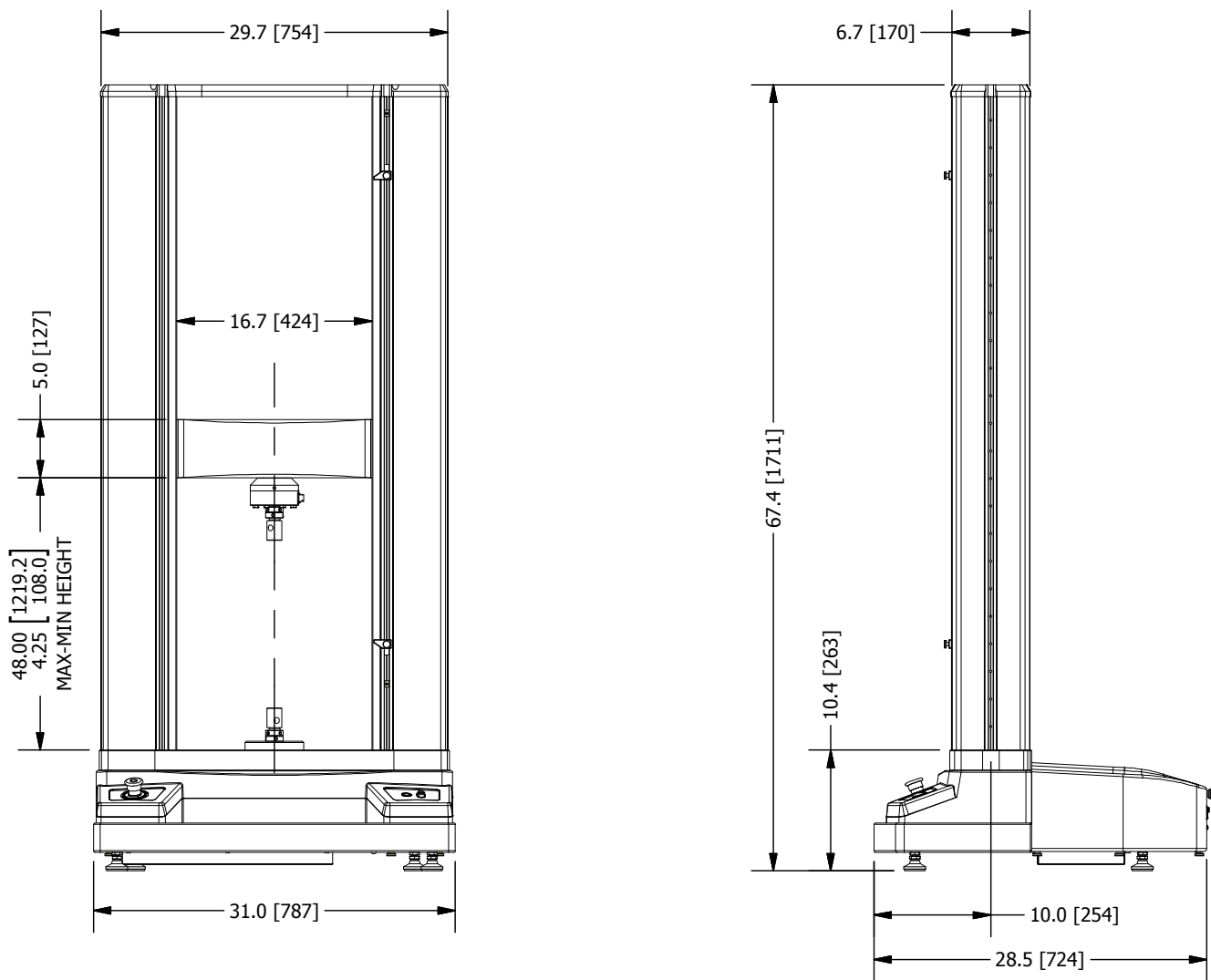
50kN Load Capacity Series Test Frames
