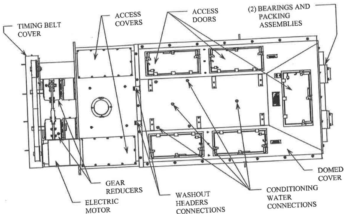
Figure 2-2. Paddle Mixer/Unloader (Top View)
