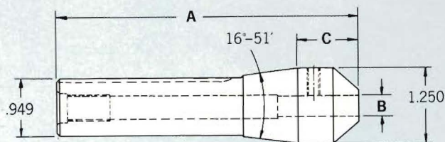
R-8 TAPER
