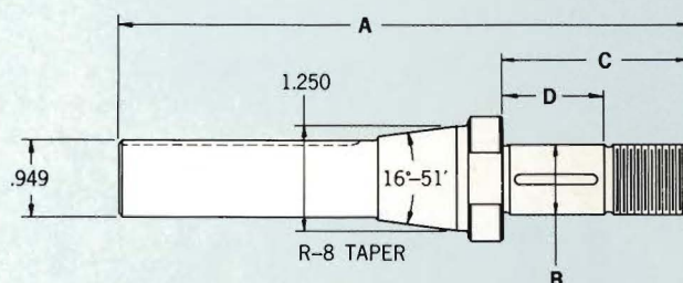
SPACERS for use with Bridgeport Stub Arbors.
