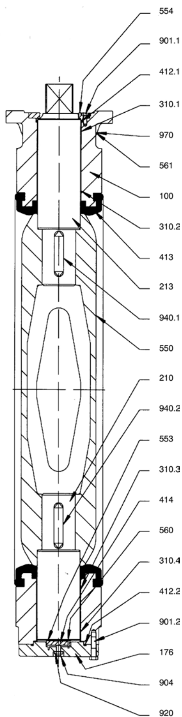
Series 280 / 400 / 520
