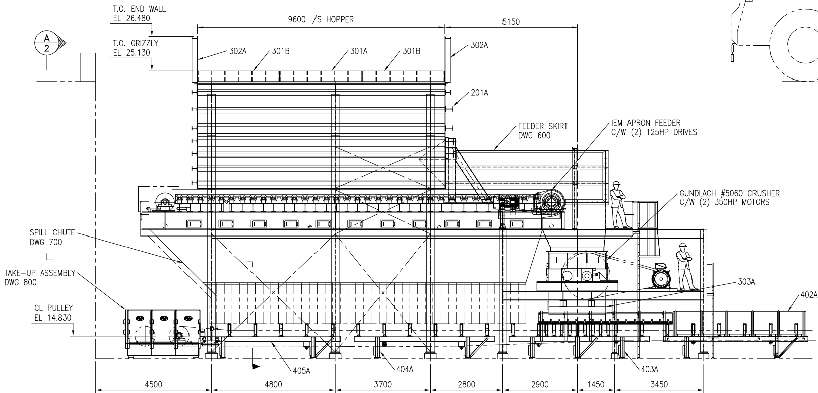
ELEVATION VIEW
